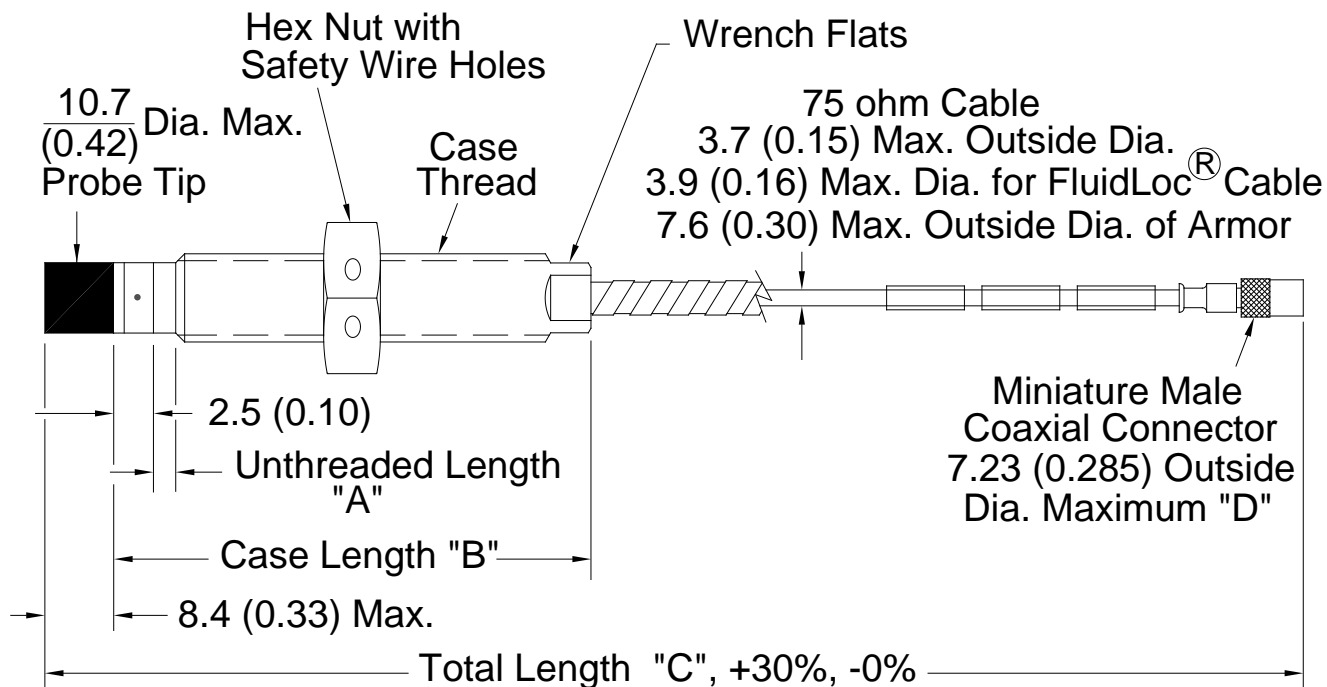
Figure 11 3300 XL 11 mm Proximity probes, Standard Mount
